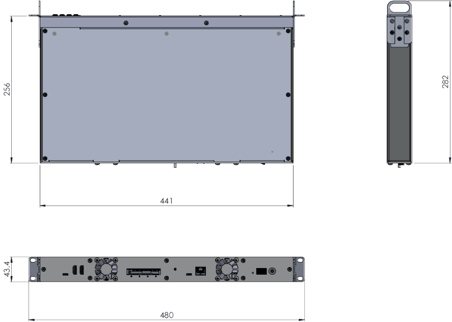
Figure 11: ACQ2106 Channel Panel Case Dimensions (mm)
