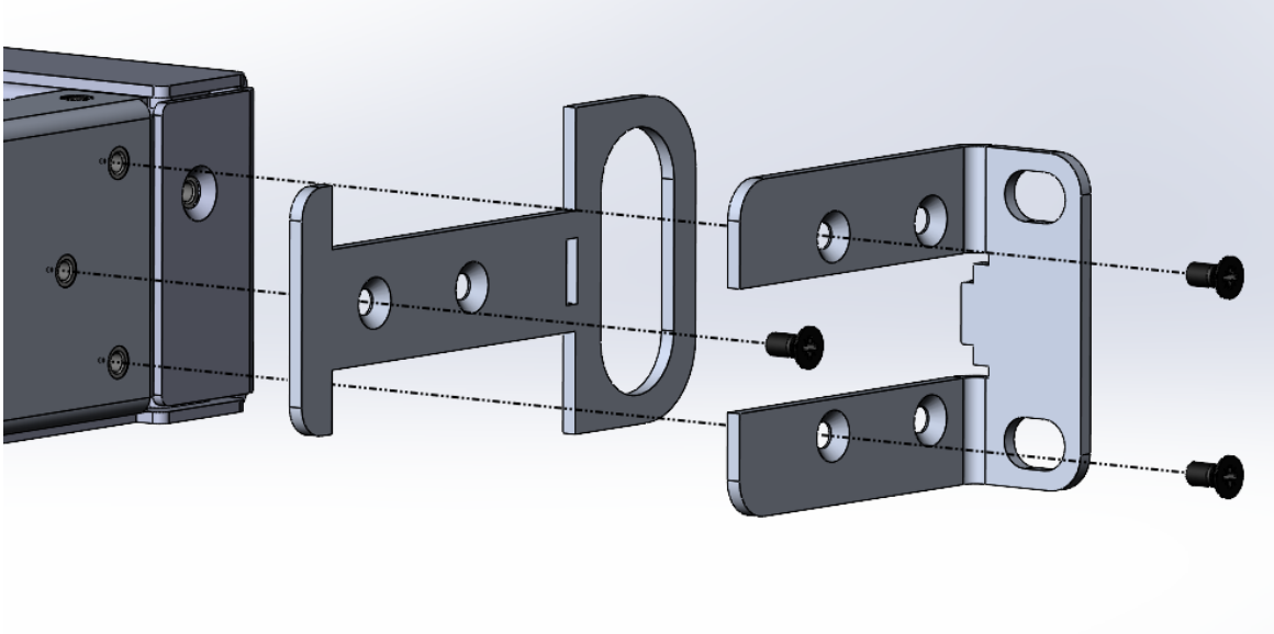
Figure 9: Channel Panel Case Rack Mount
