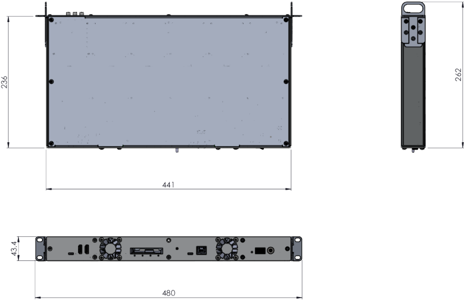
Figure 10: ACQ2106 Standard Case Dimensions (mm)
