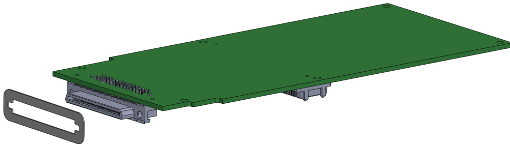
Figure 6: VHDCI Shim on ELF Module
